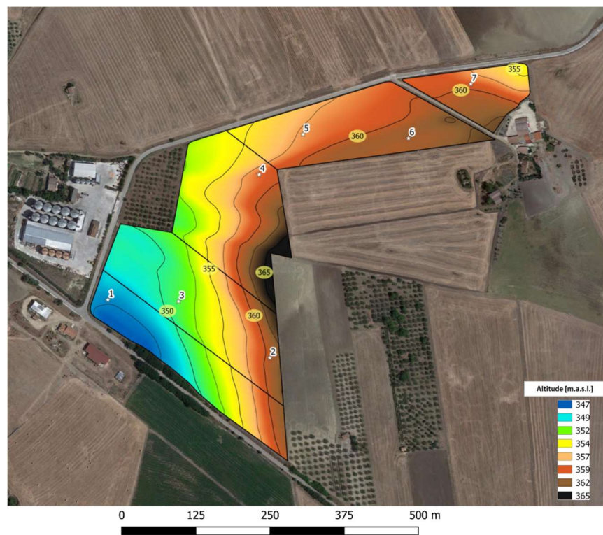
Figure 4. The altitude map of demonstration fields.
